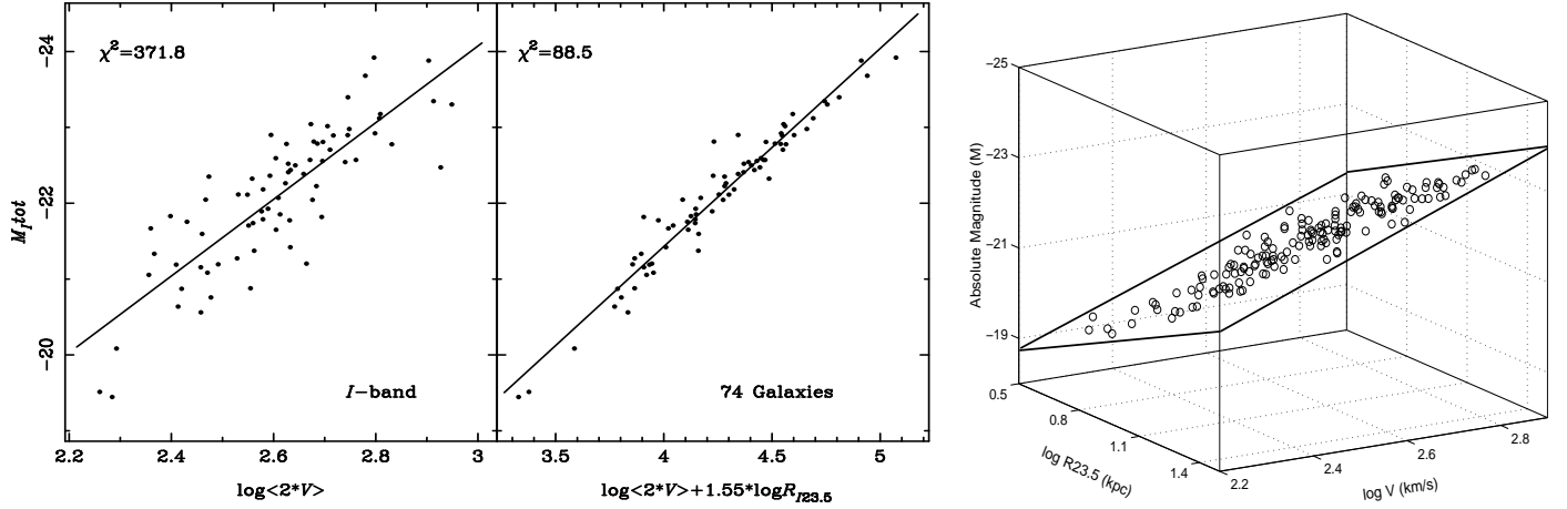
Fig. 3. Comparison of the Tully–Fisher relation (the left side) and the best-fitting plane (the right side). Data of 74 galaxies were taken from Palunas and Williams (2000). The typical rms errors of the absolute magnitudes were taken as 0.2 mag. The data distribution in 3-D space was also plotted.
